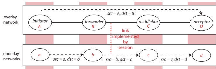
Fig. 17. A prototypical overlay session.
